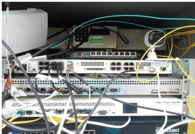
Gambar 4.1 Router
