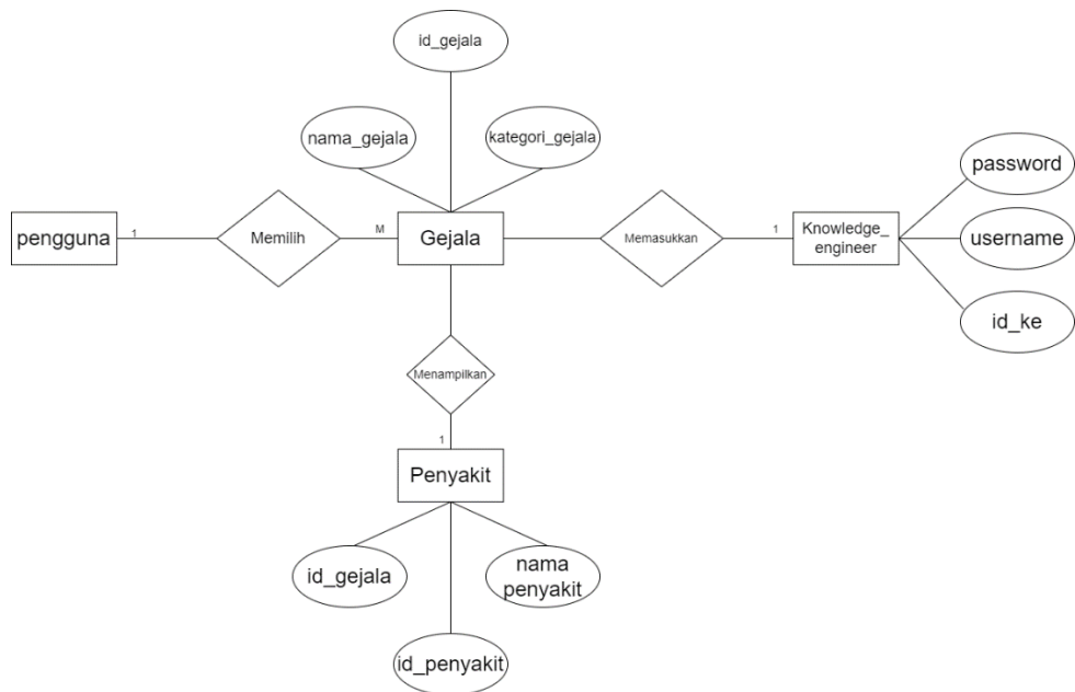
Gambar 3. 5 Entity Relationship Diagram(ERD)
