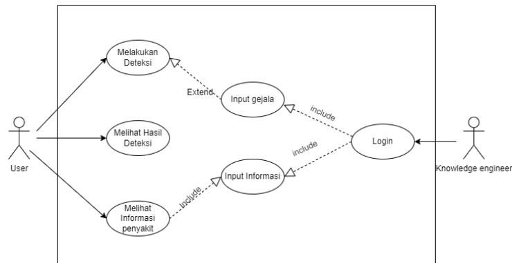
Gambar 3. 4 Use Case Diagram
