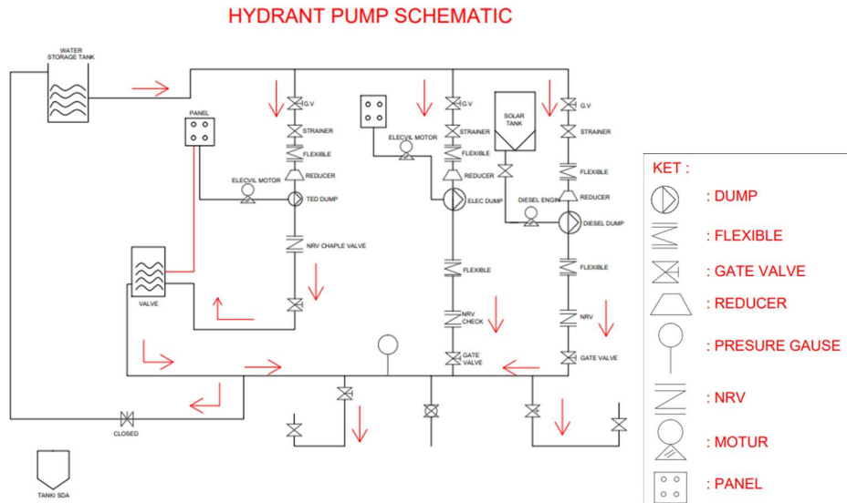
Gambar 3.2 Denah Hydrant Pump Schematic PT. Pacific Indopalm Industries Sumber : Dokumentasi KP
