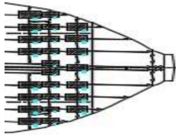
Gambar 2. 28 Titik NDT deck cargo barge
