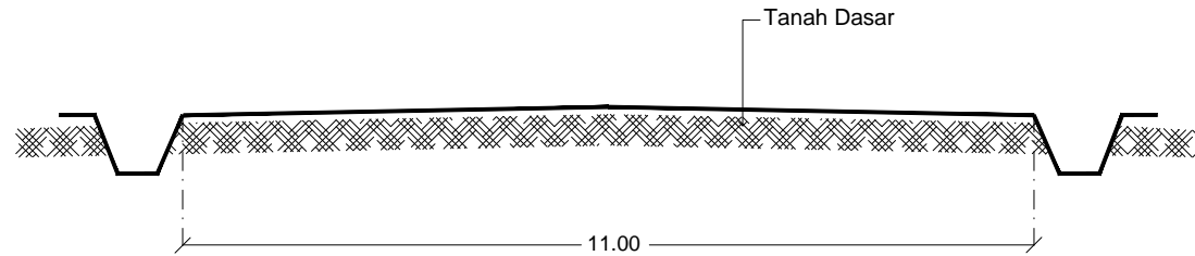
Ⓜ PENAMPANG EXISTING JALAN SECTION 1 STA 0+000
