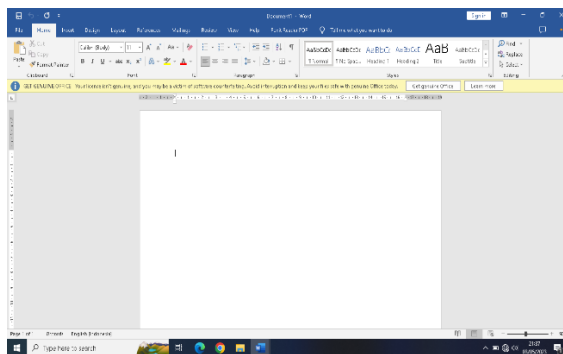
Gambar 3.5 Microsoft Word
