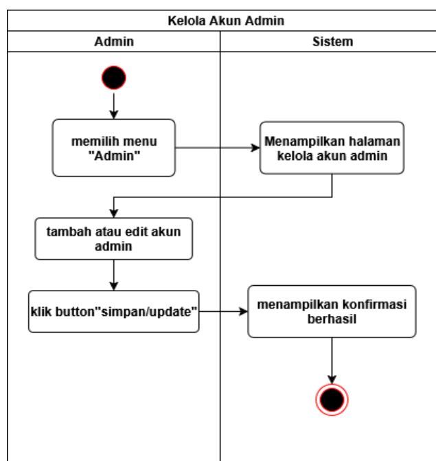
Gambar 4. 5 Activity Diagram Kelola Akun Admin
