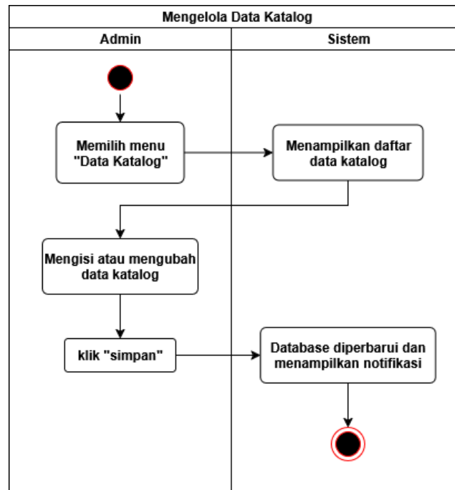
Gambar 4. 3 Activity Diagram Mengelola Data Katalog
