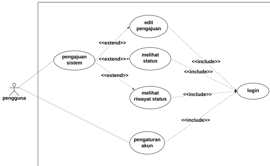
Gambar 4. 2 Use case
