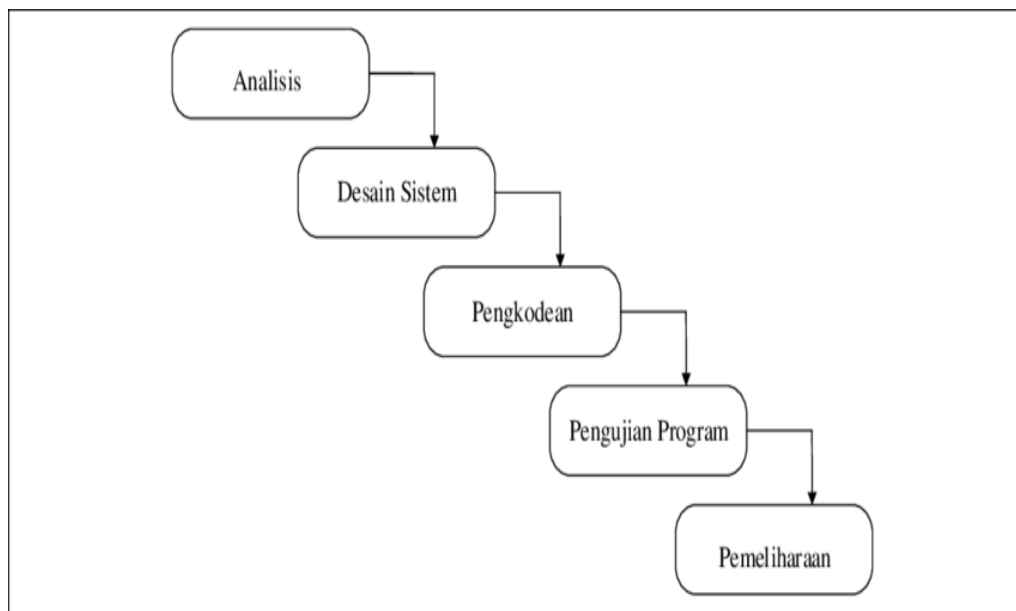
Gambar 4. 1 Metode Waterfall
