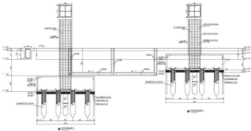
DETAIL PEMBESIAN PIT LIFT GRID 9B-C SKALA 1:35
