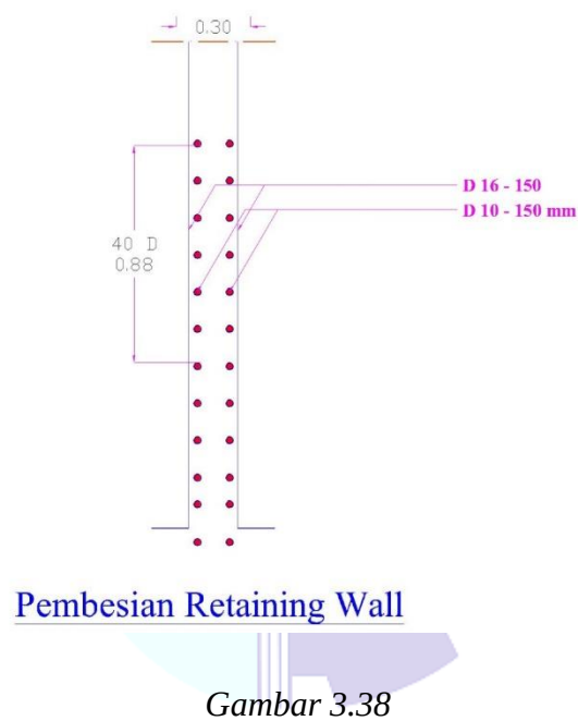
Pembesian dinding retaining wall
